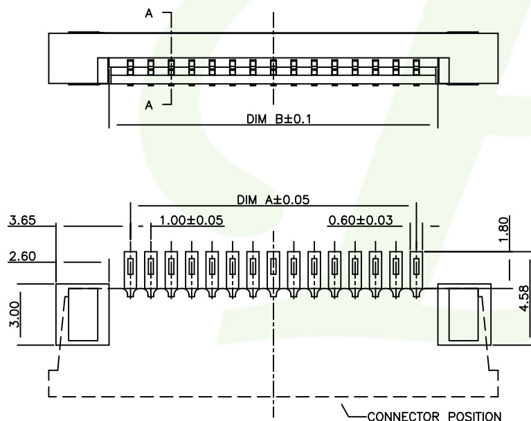
RECOMMENDED P.C.B PATTERN LAYOUT
