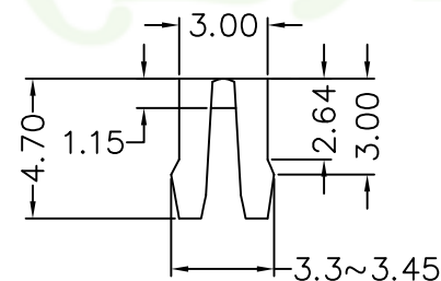
DETAIL X
