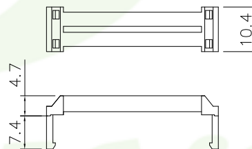
Plastic Strain Relief
