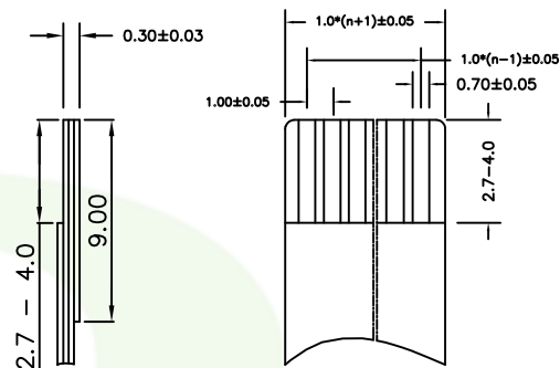
1.0mm Pitch FFC cable
