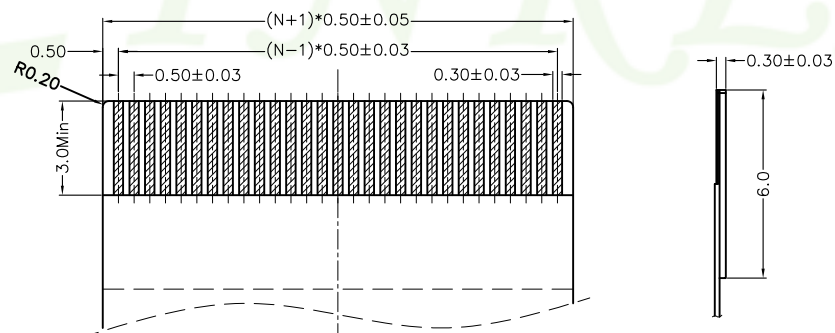
RECOMMENDED FPC/FFC DIMENSION
