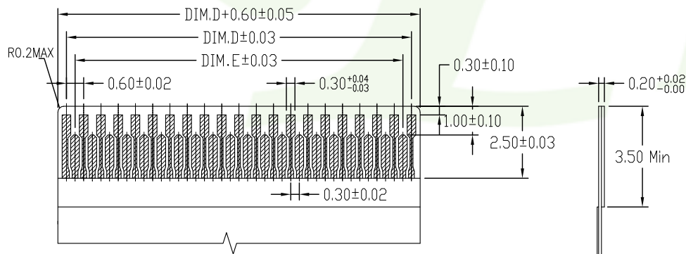
RECOMMENDED FPC DIMENSIONS
