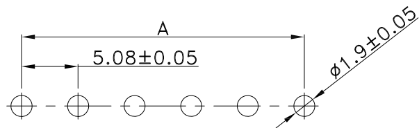
Recommant PCB Layout
