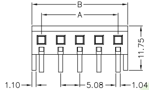
757-71-xxT (A Type)
