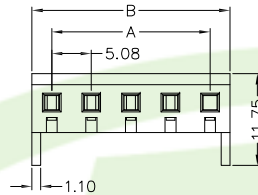
757-72-xxT (B Type)
