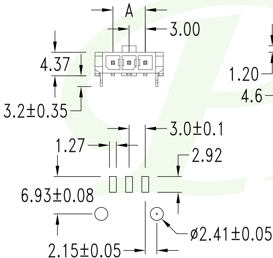
PCB Layout: Component side
