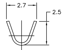
Sec. B-B
