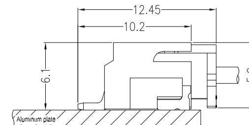
Assembly Layout
