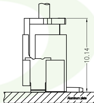
Assembly Layout
