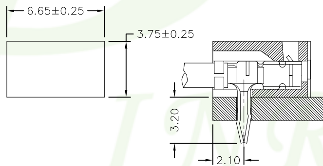
Mated Drawing(REF.)
