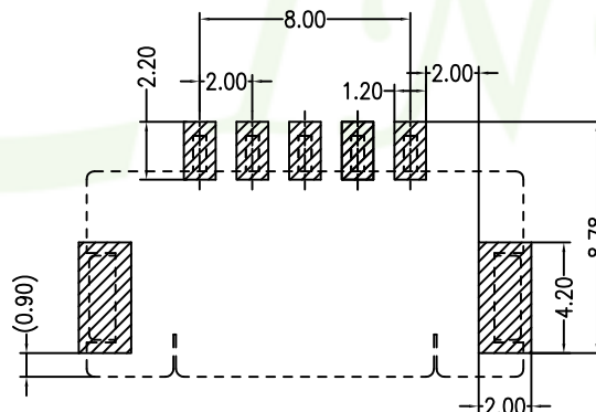
PCB LAYOUT(Tolerance:±0.05)
