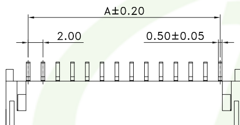
RECOMMENDED PCB LAYOUT DIM. General tolerance \pm 0.05
