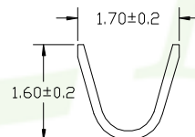
C-C SEC
