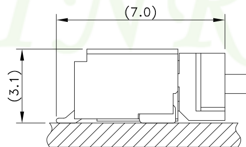
ASSEMBLED VIEW
