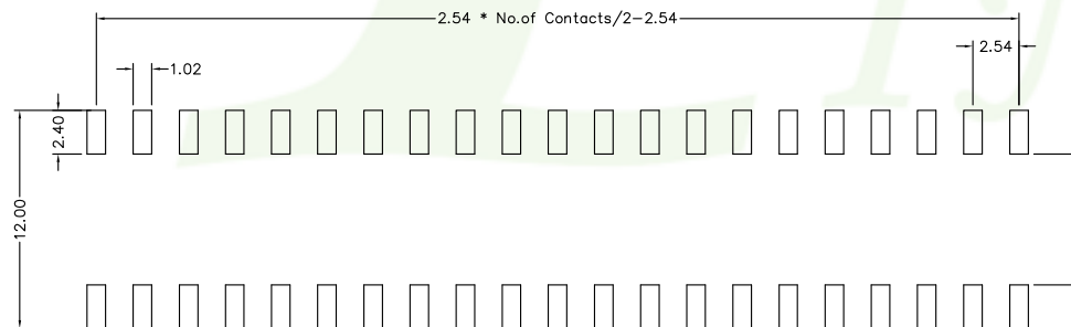
Recommended P. C .Board Hole Layout
