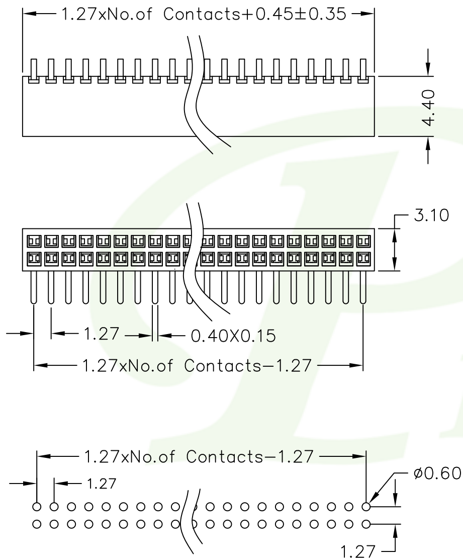
Recommended p.c. Board SMD Layout
