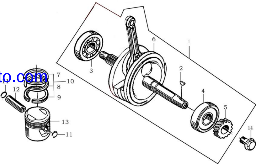
曲轴连杆部件/活塞 CRANKSHAFT CONNECTING-ROD ASSY/PISTON
