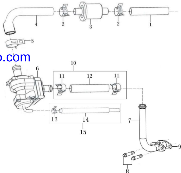
环保装置 ENVIRONMENT PROTECT MECHANISM
