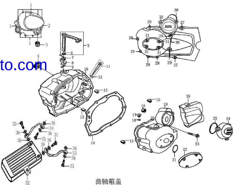
曲轴箱盖 CRANKCASE COVER
