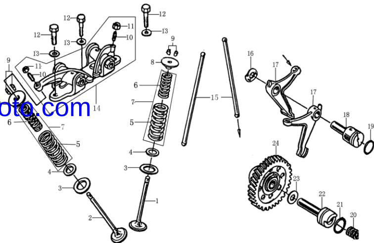
配气机构 VALVE MECHANISM
