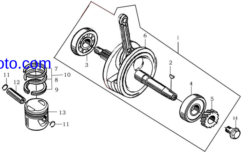
曲轴连杆部件/活塞 CRANKSHAFT CONNECTING-ROD ASSY/PISTON
