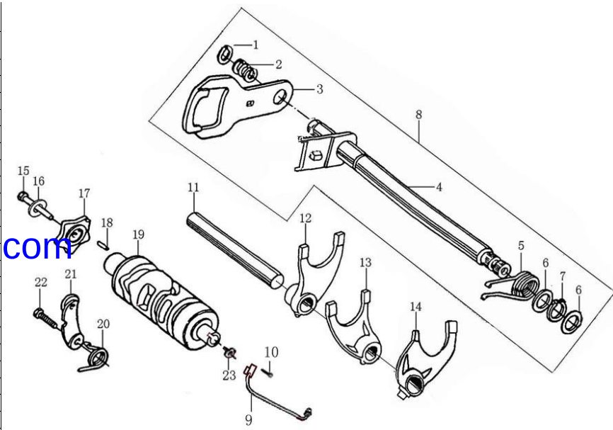
变速器 GEARSHIFT MECHANISM
