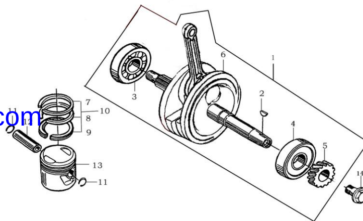
曲轴连杆部件/活塞 CRANKSHAFT CONNECTING-ROD ASSY/PISTON
