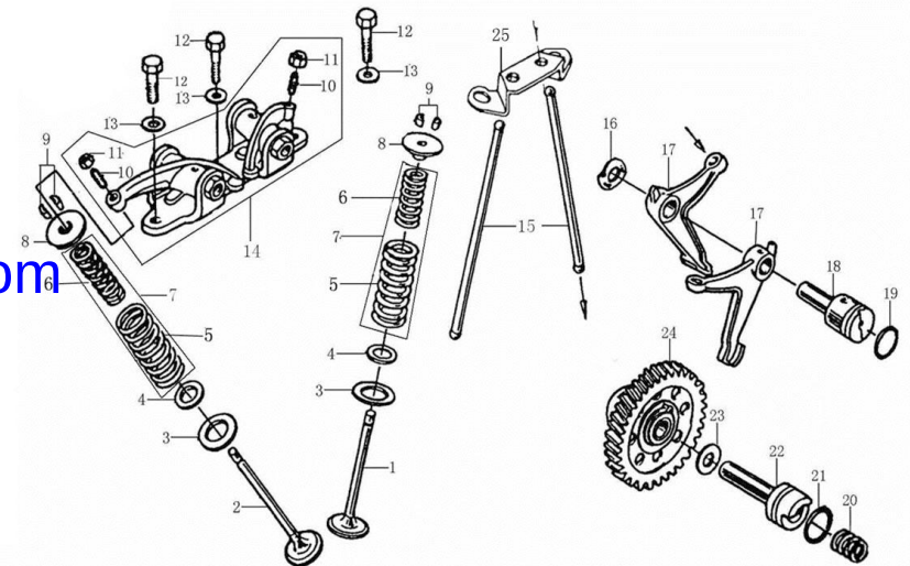
配气机构 VALVE MECHANISM
