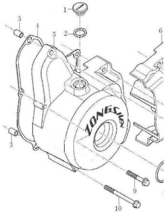
左曲轴箱盖 LEFT CRANKCASE COVER
