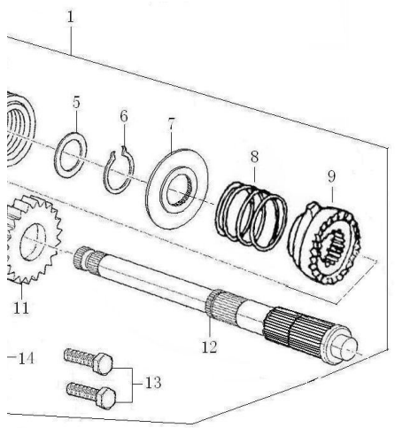
启动轴总成 STARTING SHAFT ASSEMBLY
