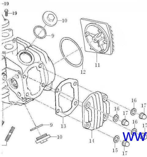
气缸头部件 LINDER HEAD ASSY
