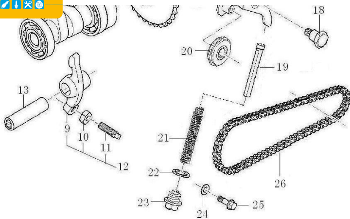
配气机构 VALVE MECHANISM
