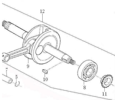
连杆部件/活塞 CONNECTING-ROD ASSY/PISTON
