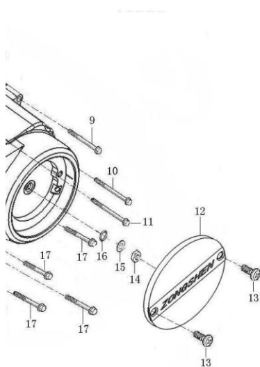
箱盖 CASE COVER
