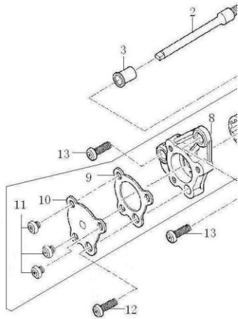
机油泵 OIL P
