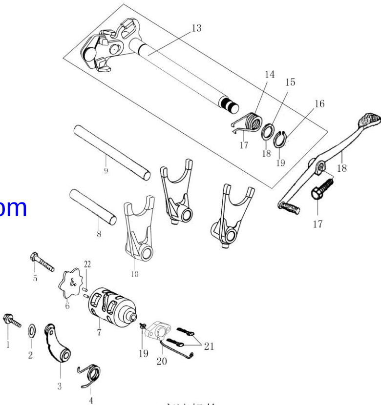
变速机构 GEARSHIFT MECHANISM
