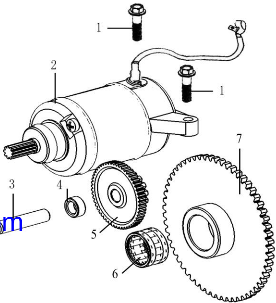
电启动机构 ELECTRIC STARTING MECHANISM
