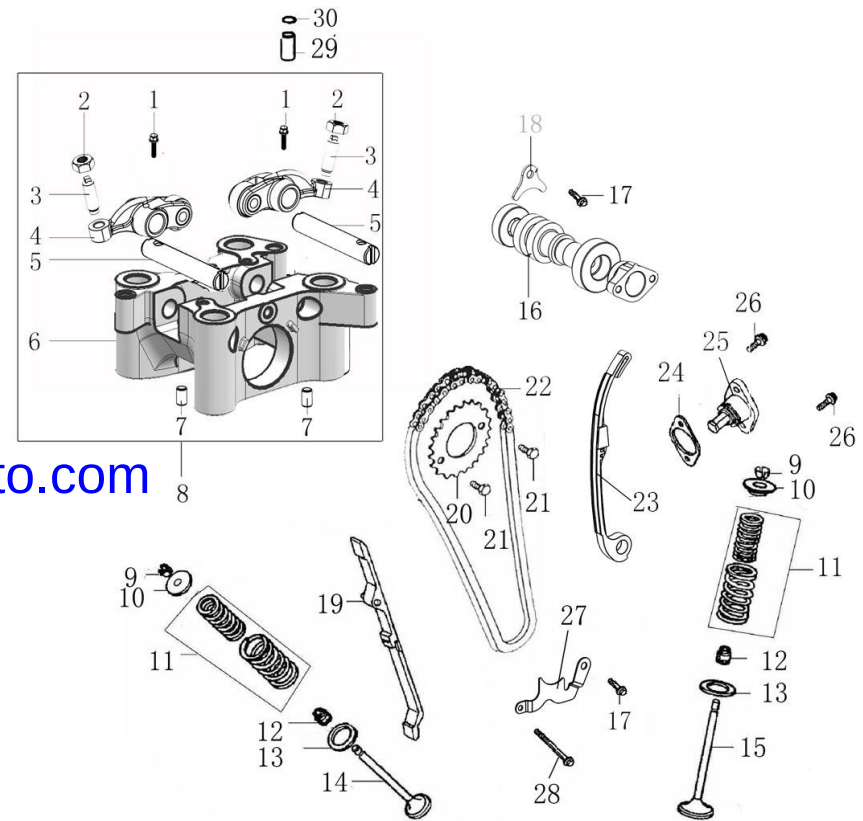
配气机构 VALVE MECHANISM
