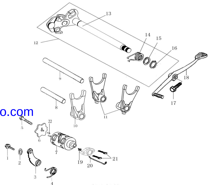
变速机构 GEARSHIFT MECHANISM
