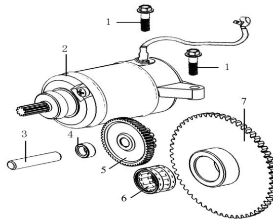
电启动机构 ELECTRIC STARTING MECHANISM
