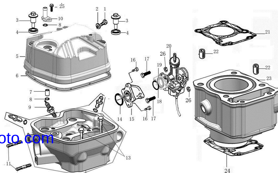
气缸头部件/气缸体部件 CYLINDER HEAD ASSY/CYLINDER ASSEMBLY
