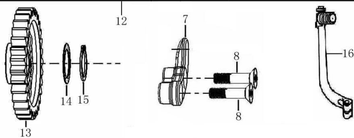
启动轴总成 KICK STARTING SHAFT ASSEMBLY
