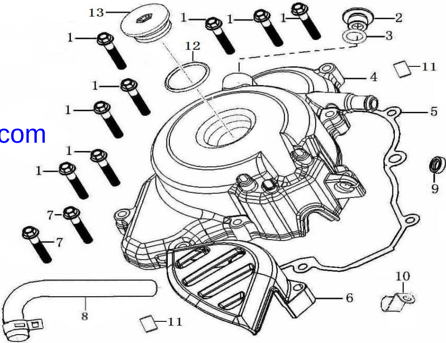
左曲轴箱盖 LEFT CRANKCASE COVER
