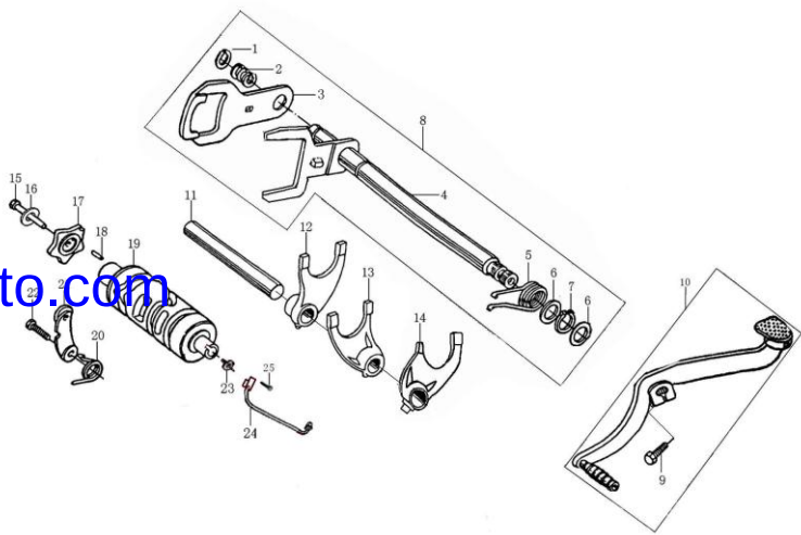
变速机构 GEARSHIFT MECHANISM
