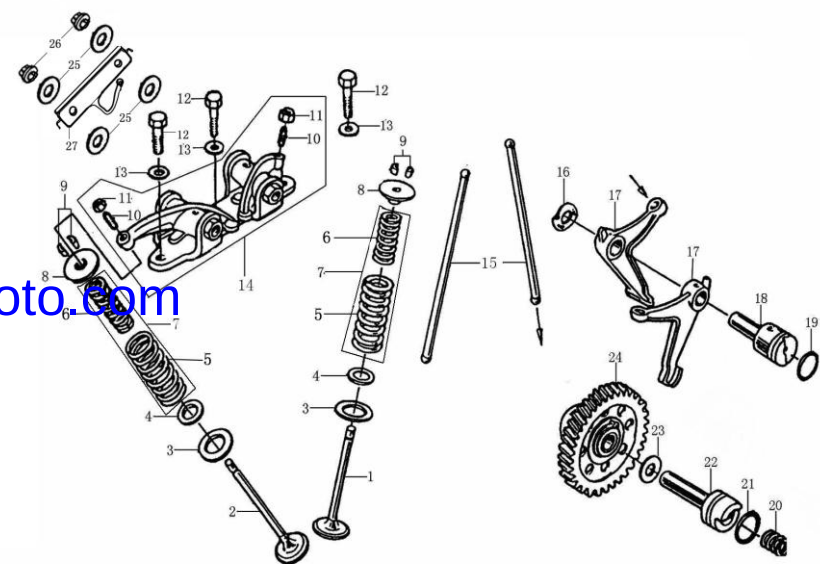
配气机构 VALVE MECHANISM
