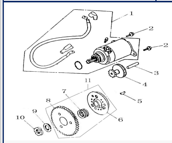
FIGURA N°28: STARTER
