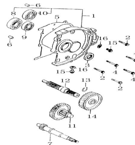
FIGURA N°21: TRANSMISION
