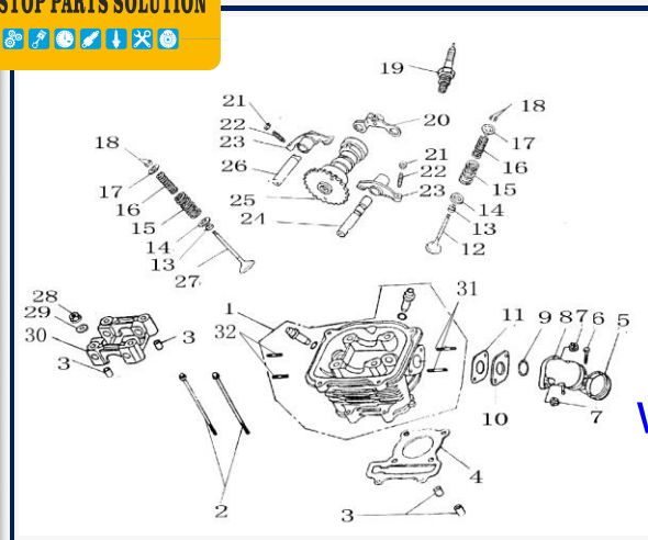
FIGURA N°25: CULATA
