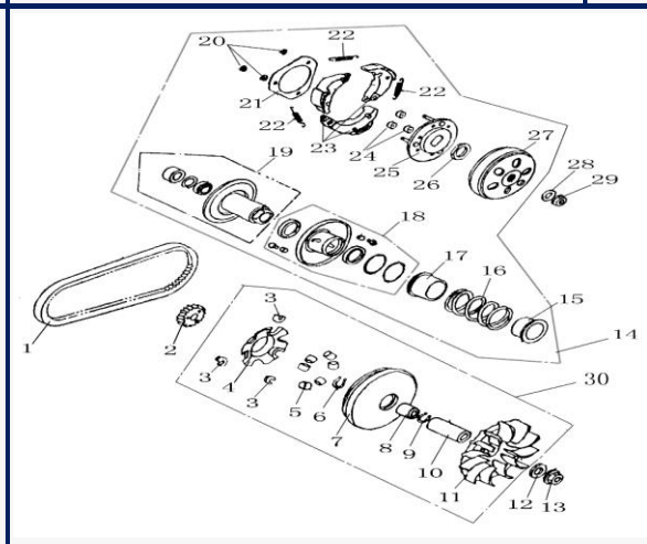
FIGURA N°29: CLUTCH
