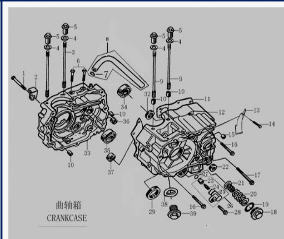
FIGURA N°21: CARTER
