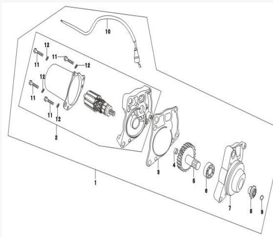
FIGURA N°17: STARTER
