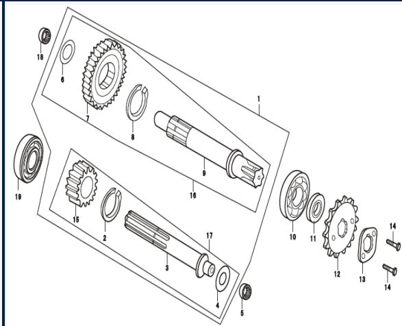
FIGURA N°15: TRANSMISION
