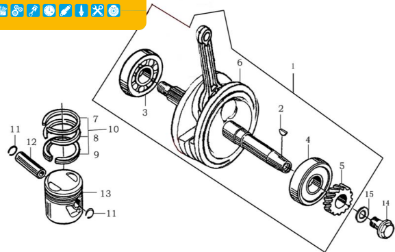
曲轴连杆部件/活塞 CRANKSHAFT CONNECTING-ROD ASSY/PISTON
