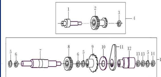
倒档惰轮机构IDLER SETUP
