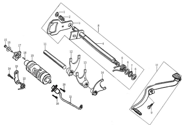
变速机构 GEARSHIFT MECHANISM
