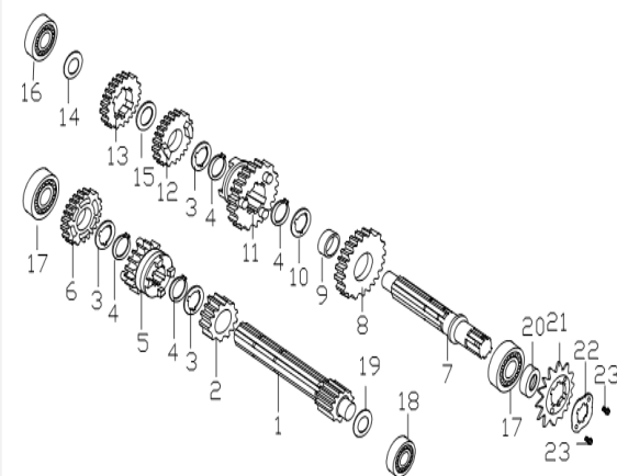
Figura N° 10: Transmission
