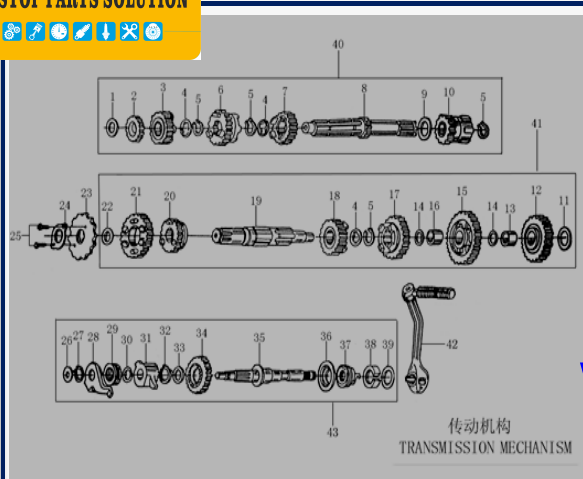
FIGURA N°25: TRANSMISION
