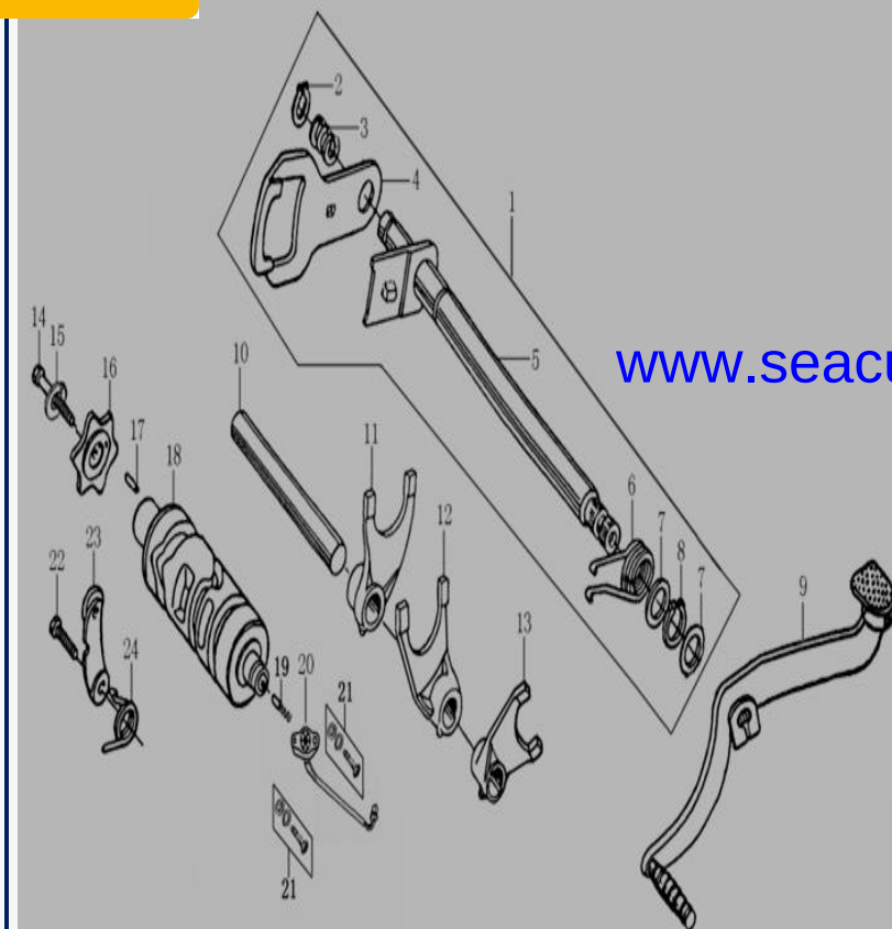
变速机构 GEARSHIFT MECHANISM
