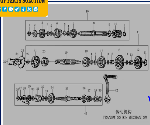
FIGURA N°25: TRANSMISION
