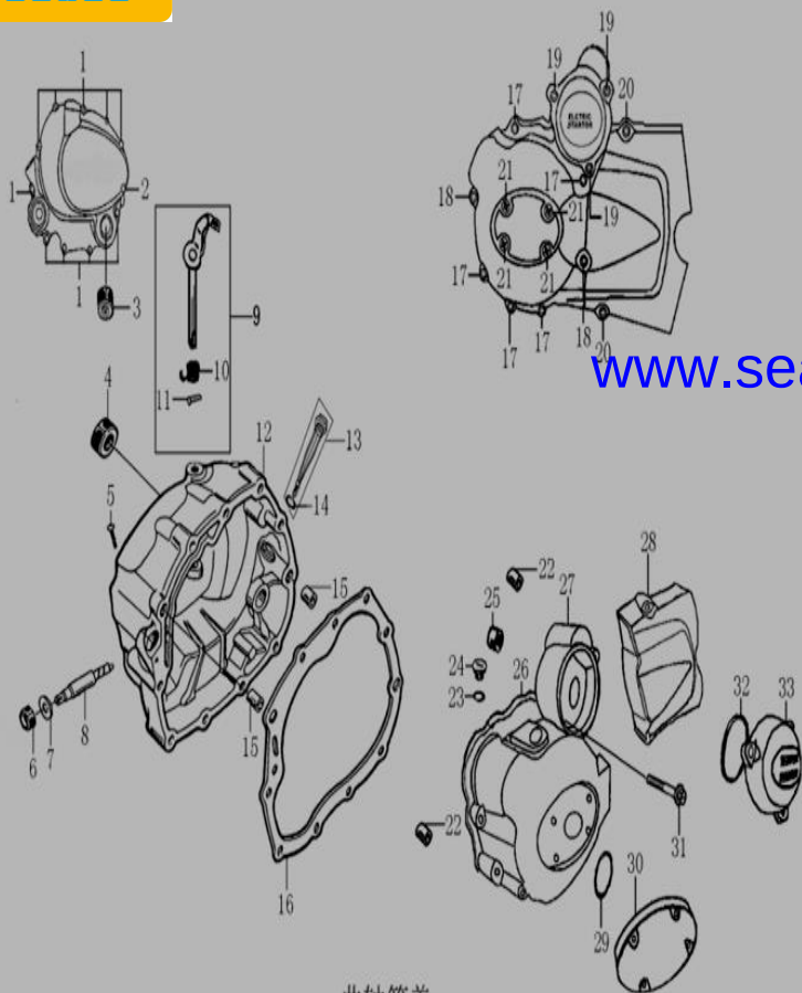
曲轴箱盖 CRANKCASE COVER
