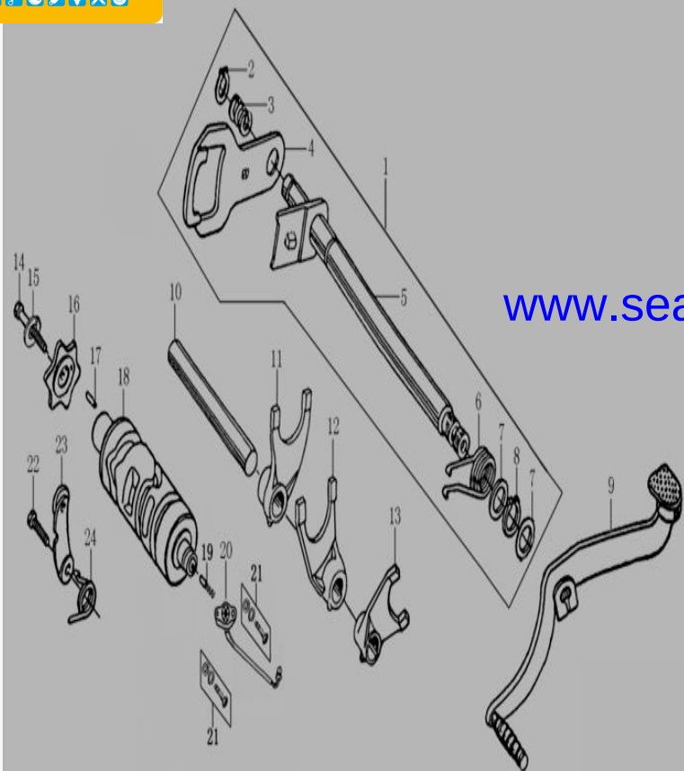
变速机构 GEARSHIFT MECHANISM
