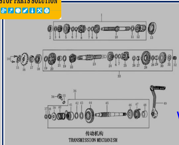
FIGURA N°25: TRANSMISION
