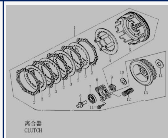
FIGURA N°21: CLUTCH
