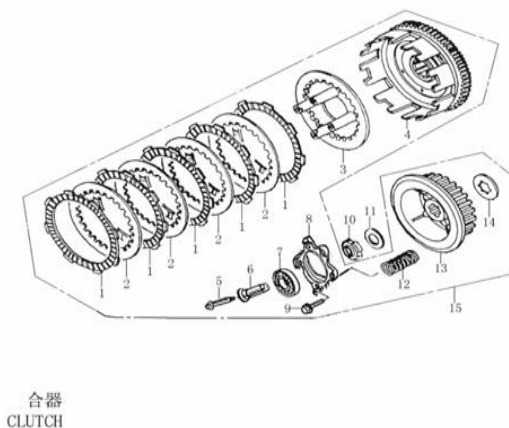
FIGURA N°21: CLUTCH
