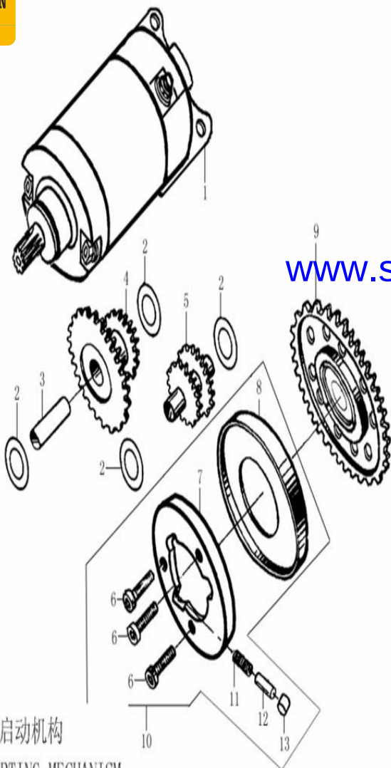
ELECTRIC STARTING MECHANISM
