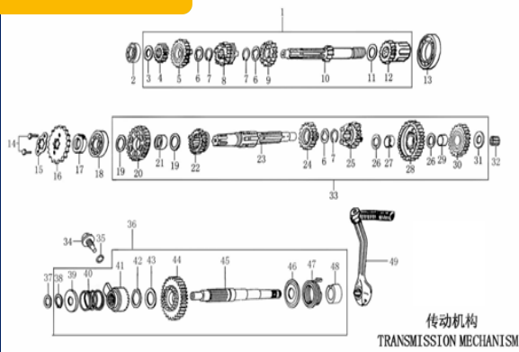
FIGURA N°25: TRANSMISSION
