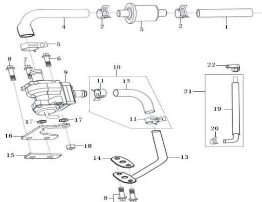
环保装置 ENVIRONMENT PROTECT MECHANISM
