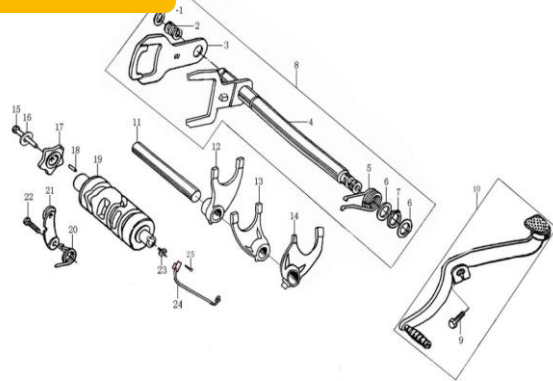
变速机构 GEARSHIFT MECHANISM
