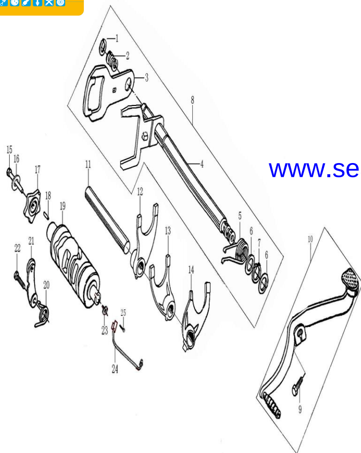
变速机构 GEARSHIFT MECHANISM
