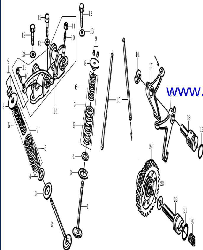
配气机构 VALVE MECHANISM
