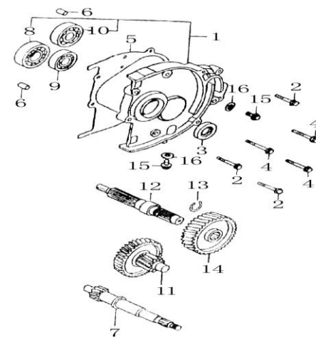
FIGURA N°21: TRANSMISION
