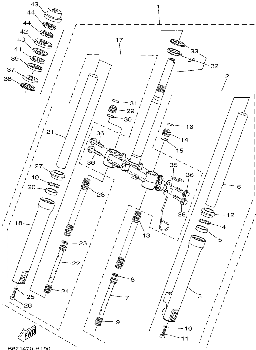
FIG.35 FRONT FORK 2 www.securemotor.com 2. ILLUSTRATION CORRECTION
