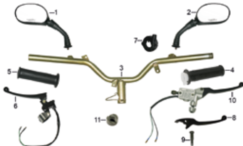
MANUBRIO F-10
