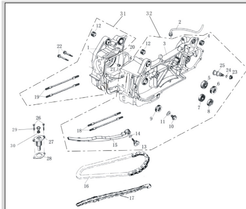
FIG 1 - CRANK CASE
