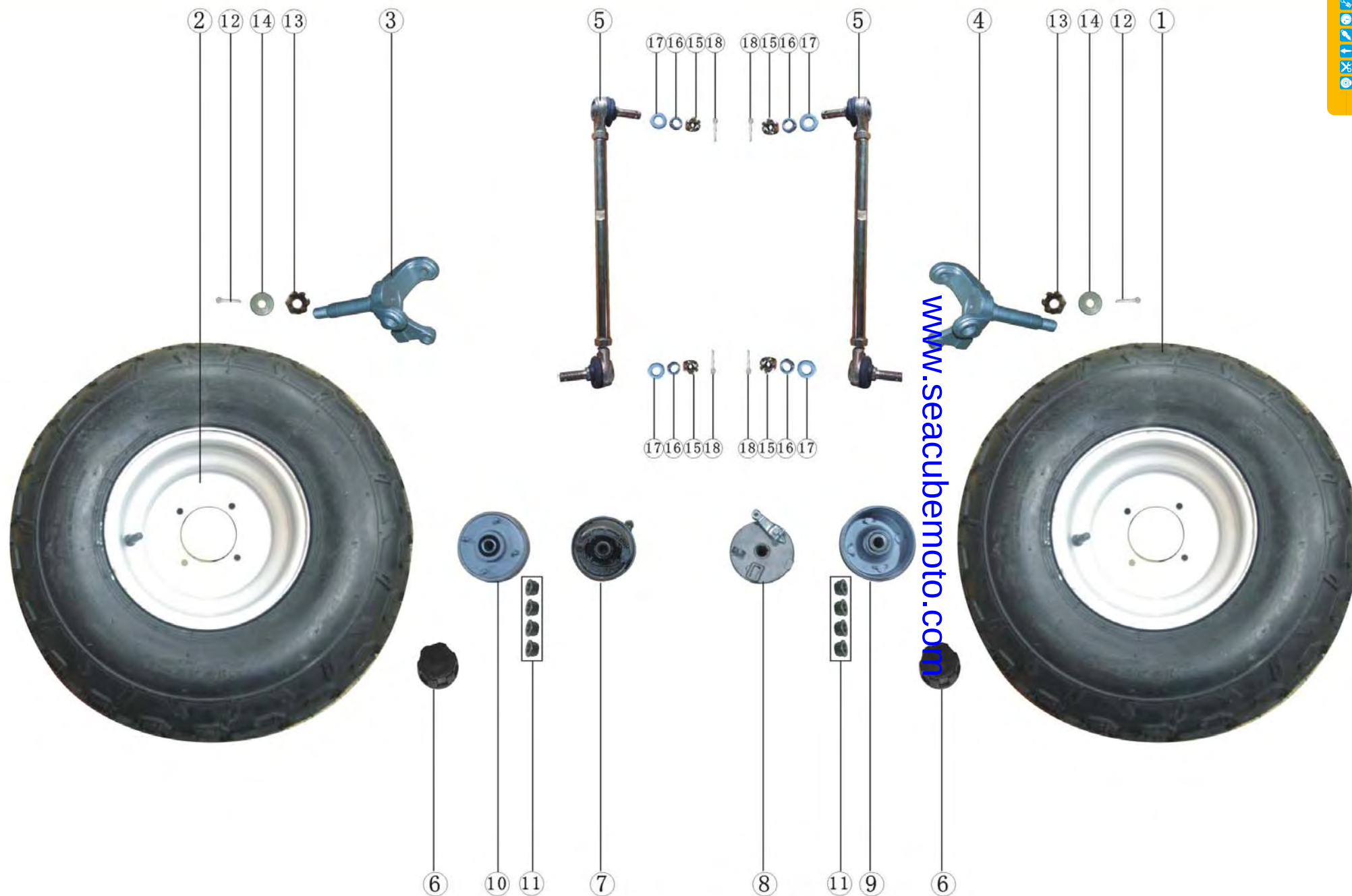
FRONT WHEEL ASSEMBLY (5)
