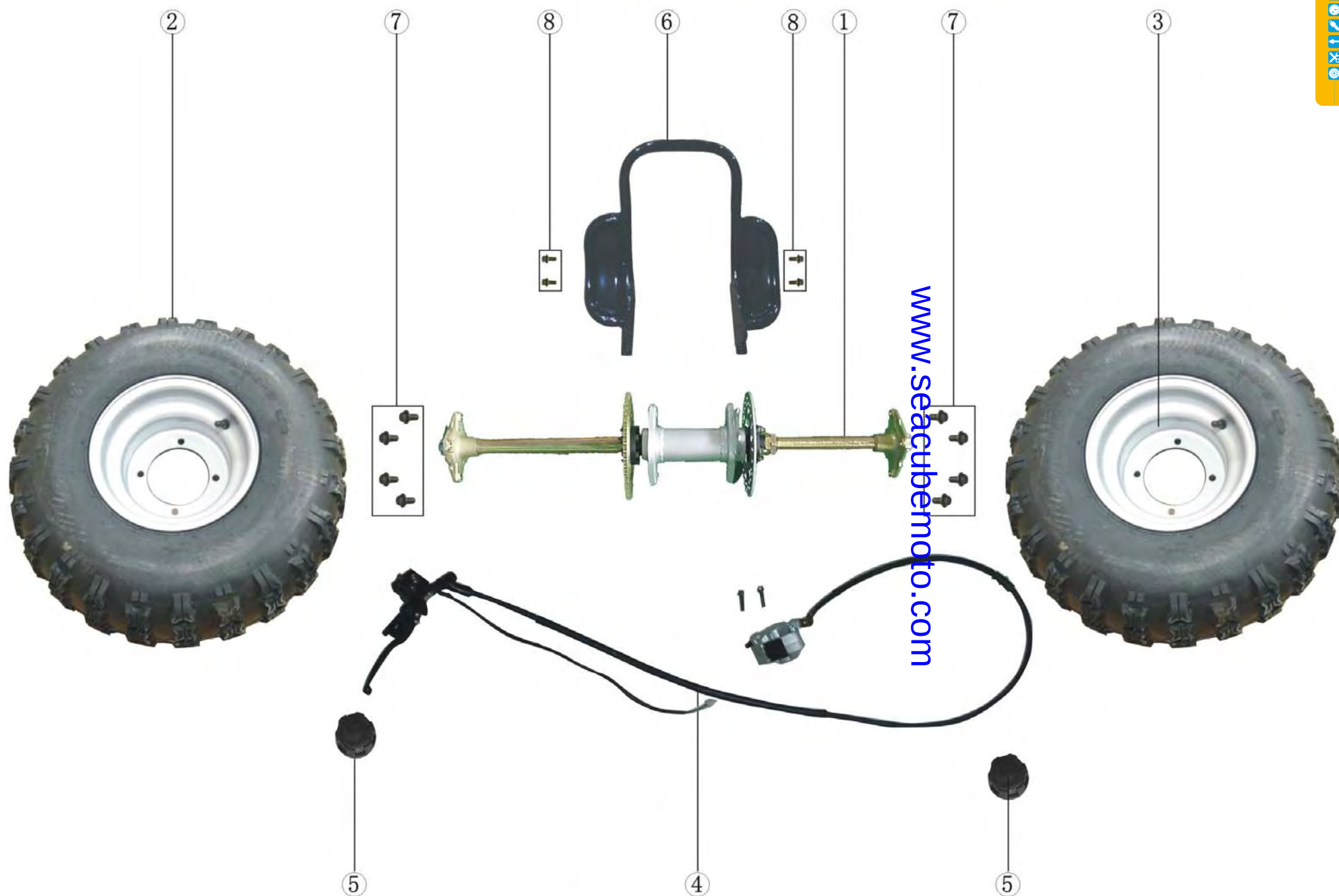
REAR WHEEL ASSEMBLY (4)
