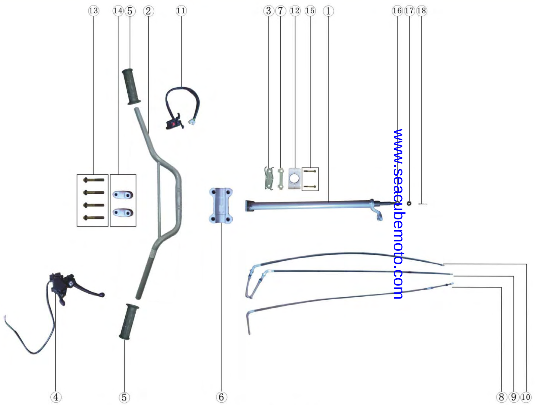
FRONT FORK ASSEMBLY (6)
