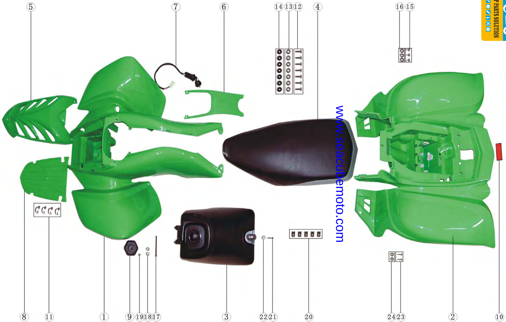
COVERING PARTS ASSEMBLY (3)
