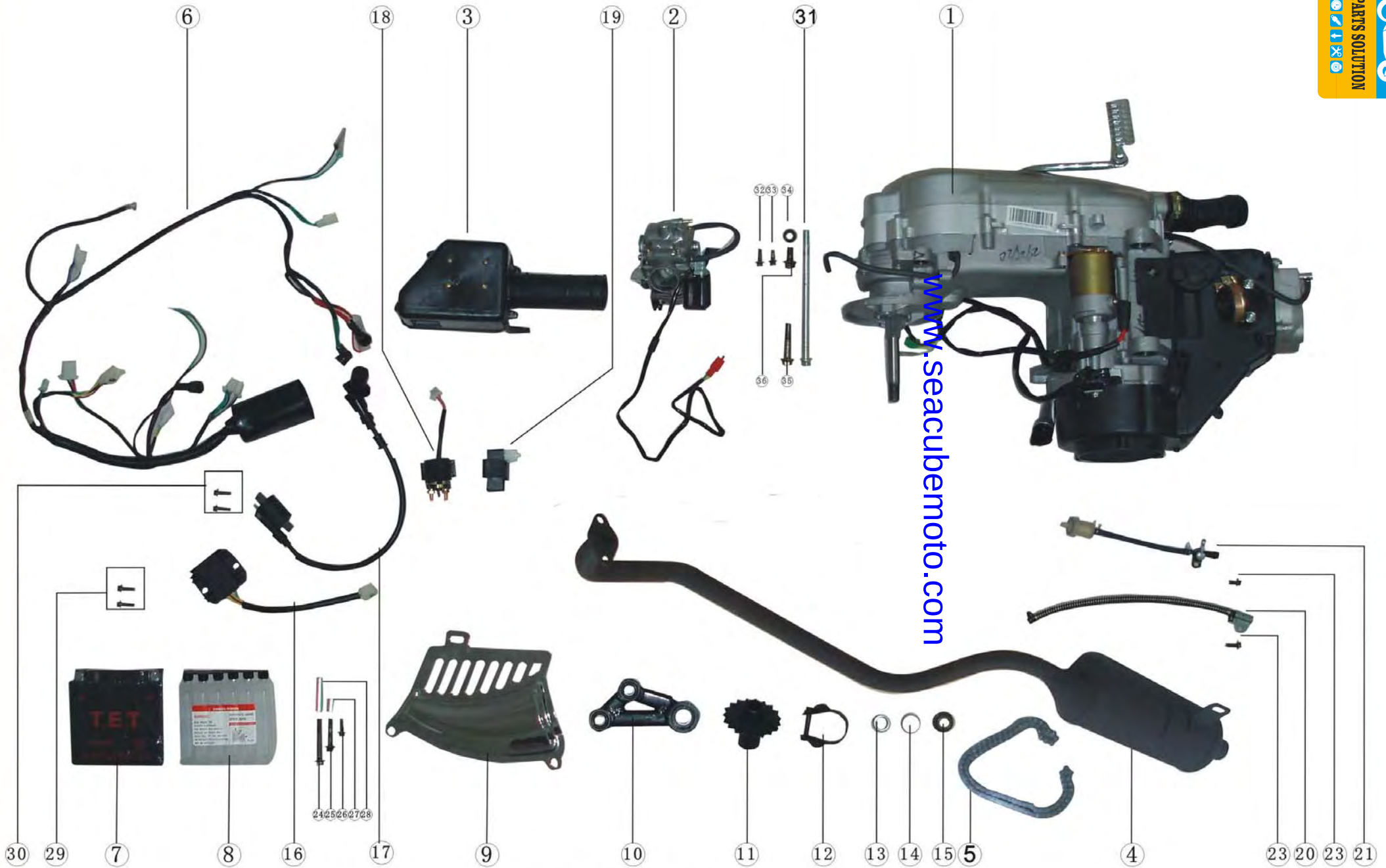
ENGINE & WIRING ASSEMBLY (2)
