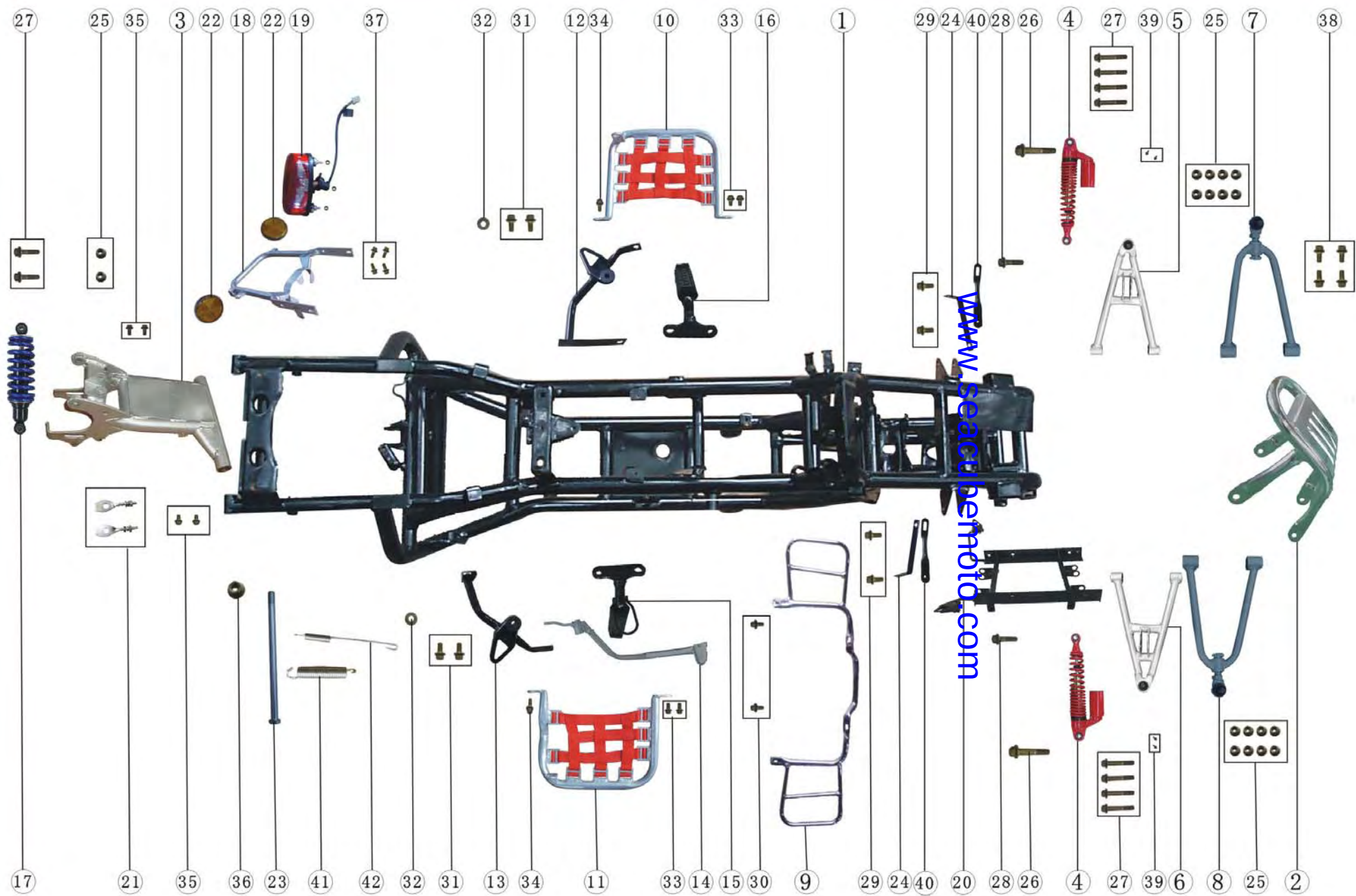
FRAME ASSEMBLY (1)
