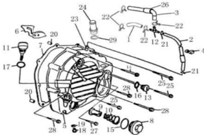
右侧曲盖总成 RIGHT CRANKCASE COVER
