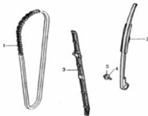
□□□□ CAM CHAIN
