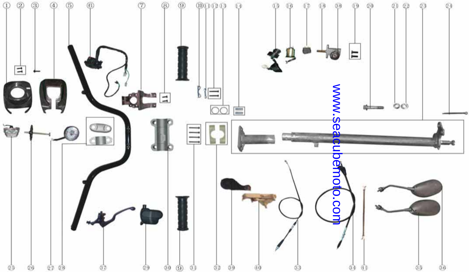
FRONT FORK ASSEMBLY (6)
