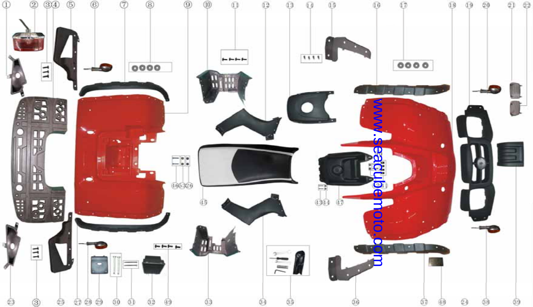
COVERING PARTS ASSEMBLY (3)
