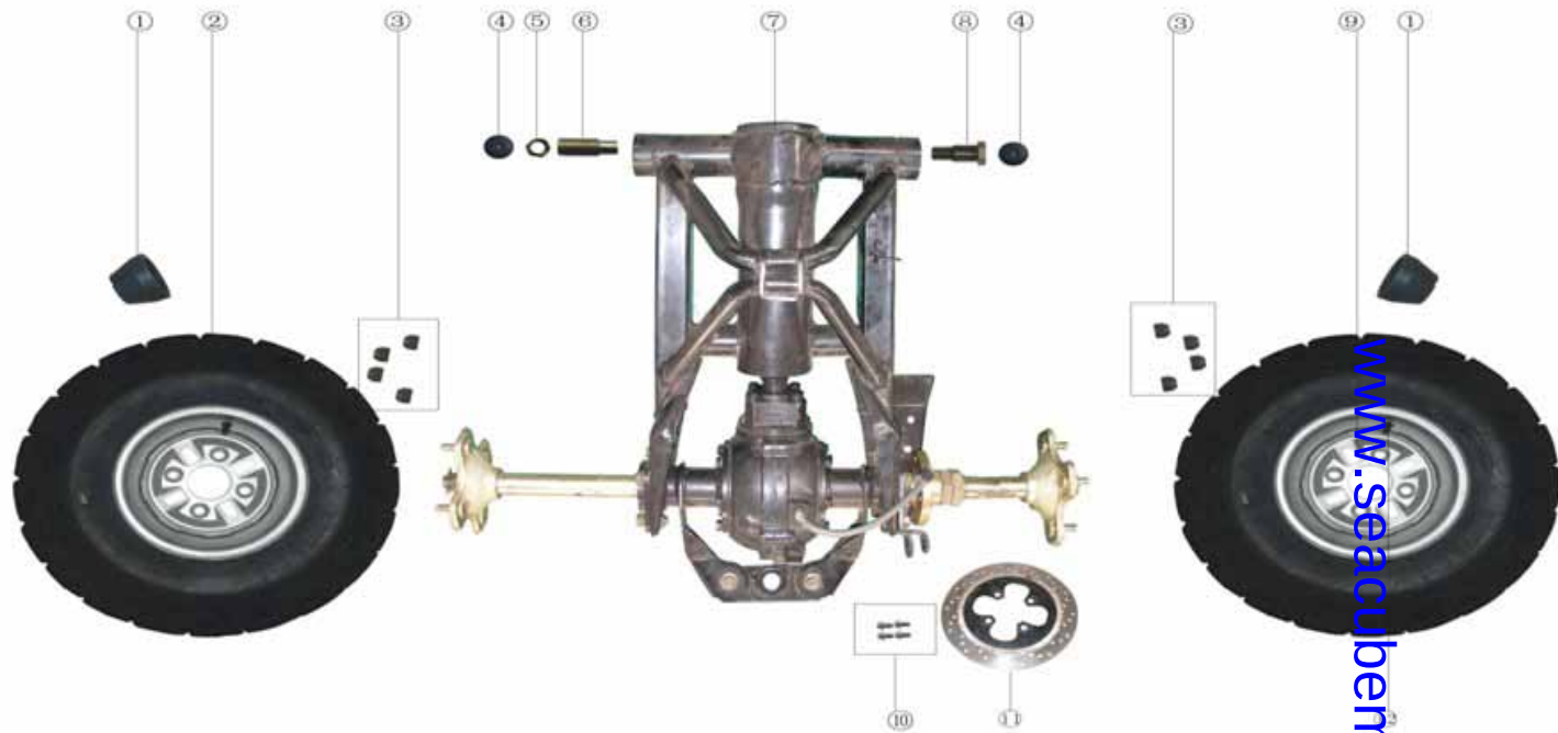
REAR WHEEL ASSEMBLY (4)
