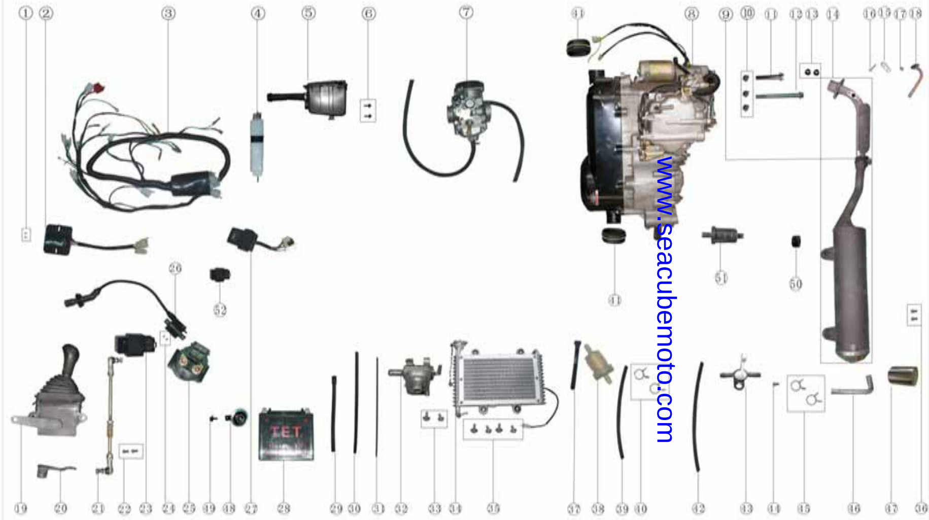
ENGINE & WIRING ASSEMBLY (2)
