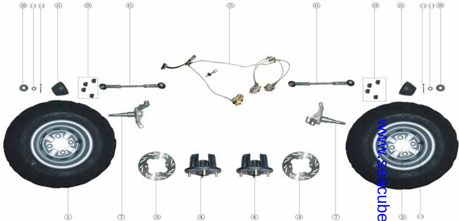
FRONT WHEEL ASSEMBLY (5)
