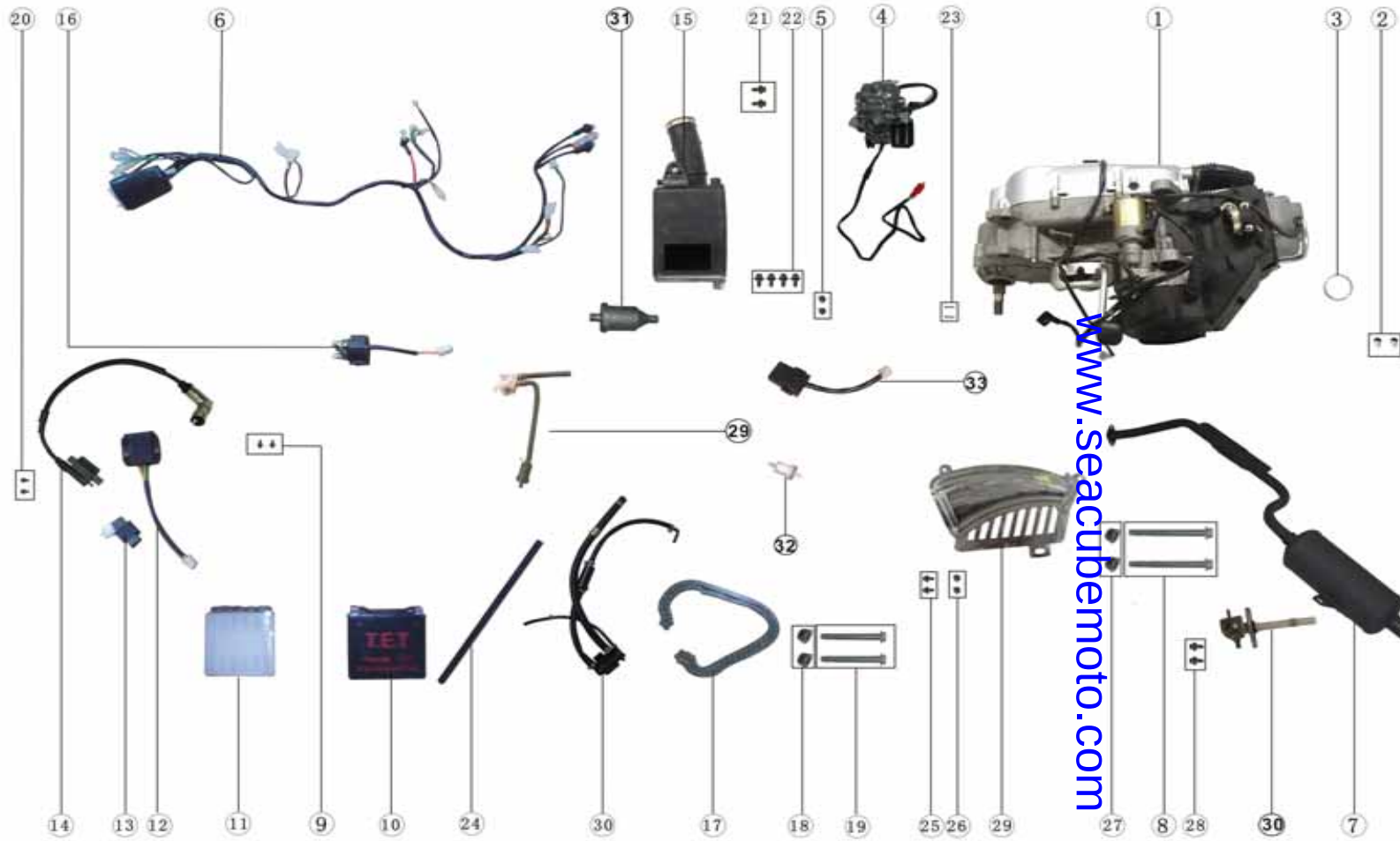
ENGINE & WIRING ASSEMBLY (2)
