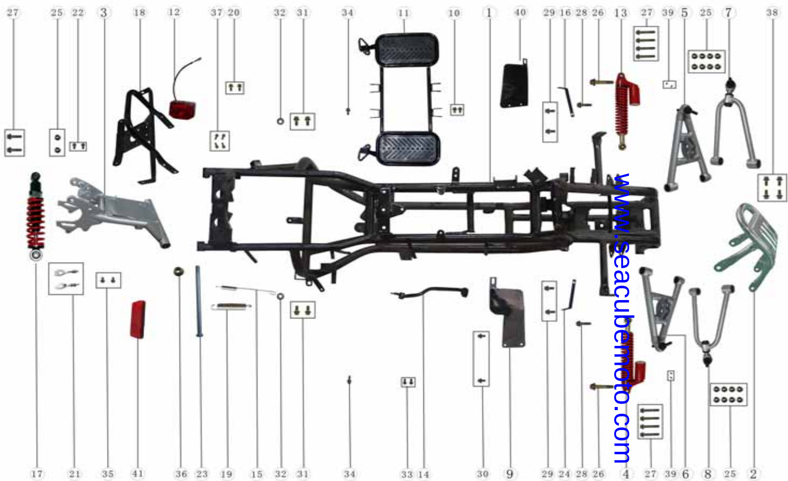
FRAME ASSEMBLY (1)
