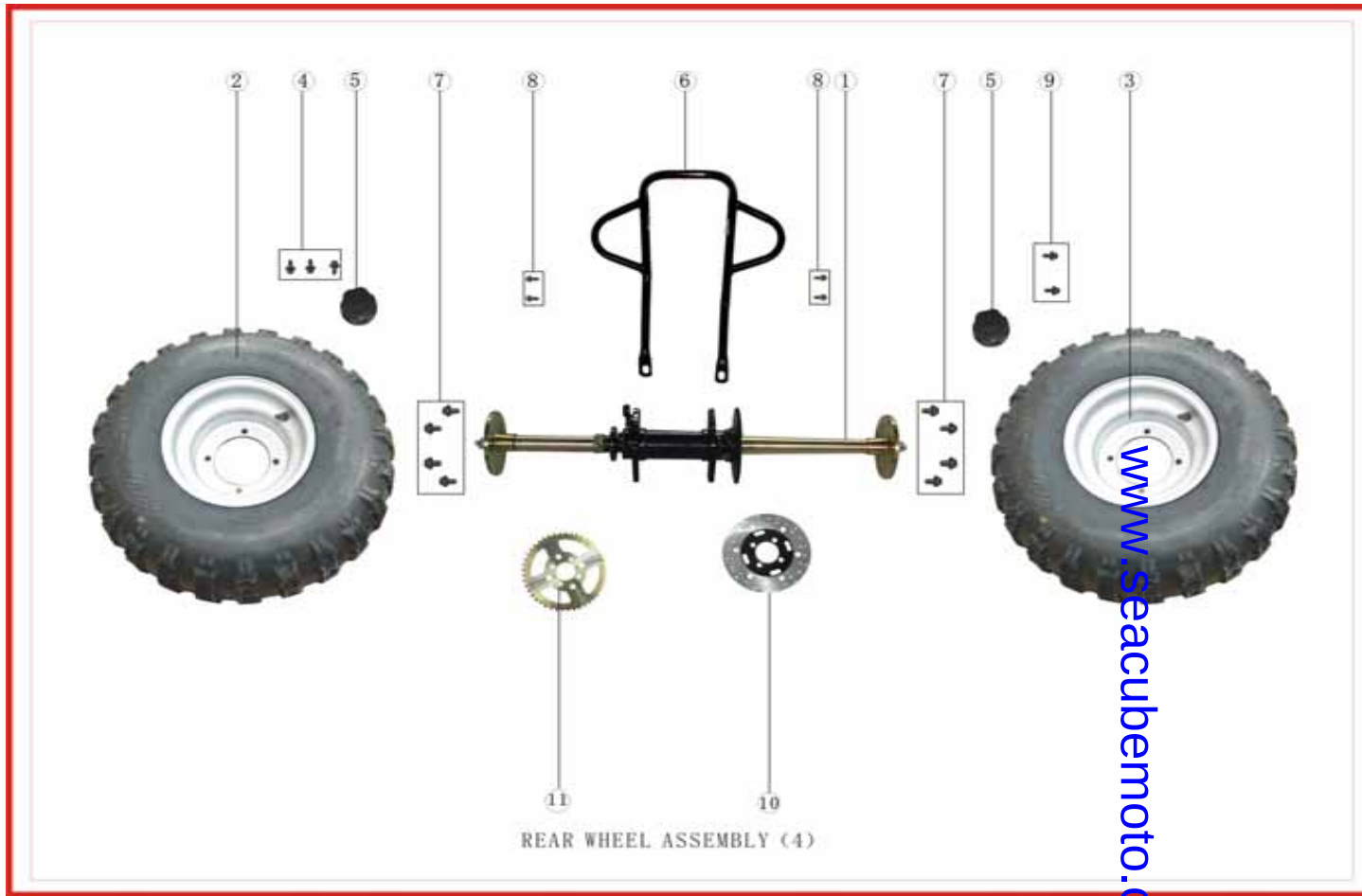
4.REAR WHEEL ASSEMBLY
