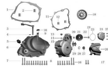
FIG 3 TAPA EMBRAGUE,VOLANTE PIÑON ,BENDIX
