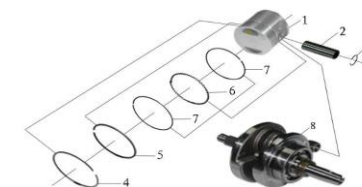
FIG.9 KIT PISTON, CIGUEÑAL
