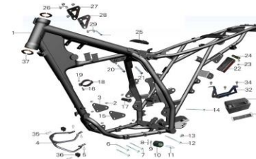
FIG.12 CHASIS,DESCANSAPIES
