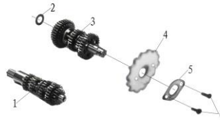
FIG.14 TRANSMISION.
