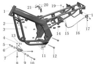
FIG.32 CHASIS
