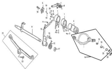
FIG.13 SELECTOR CAMBIOS
