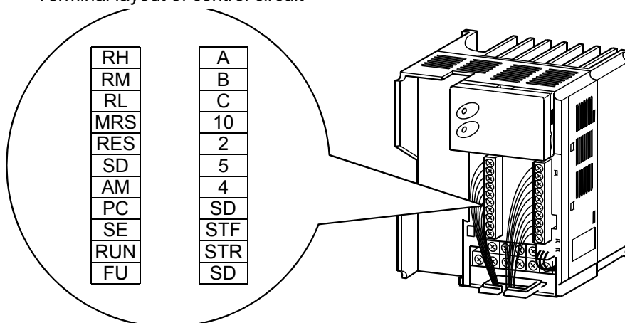
Terminal layout of control circuit
