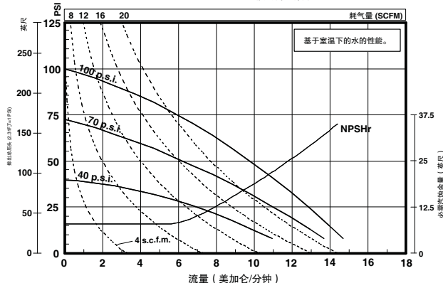
PD05P-XXX-XXX-B 1/2" 非金属隔膜泵
