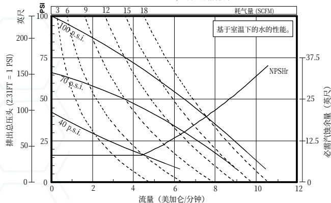
PD03P-XXX-XXX-B 3/8" 非金属隔膜泵
